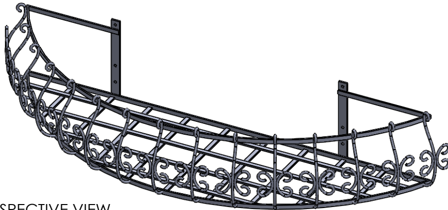
PERSPECTIVE VIEW
