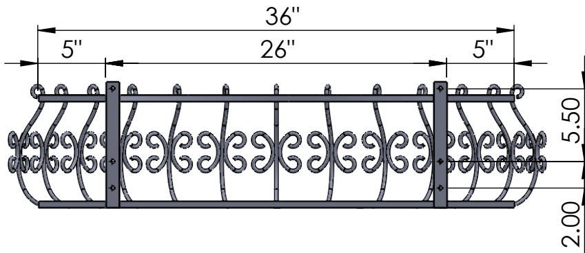
BACK VIEW
